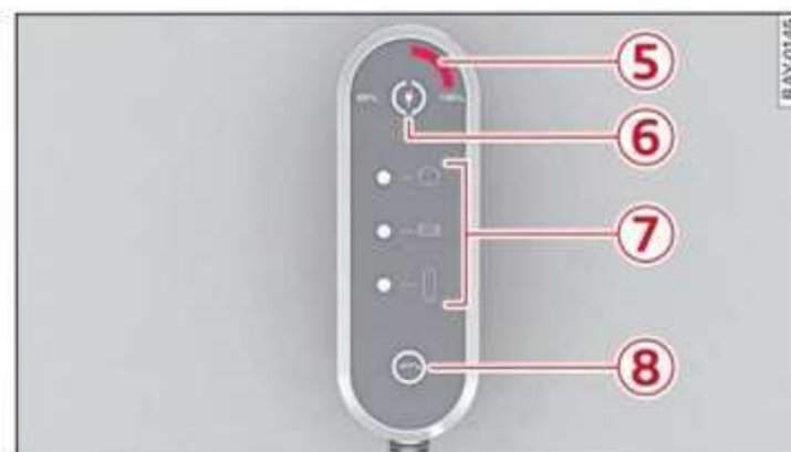
Fig. 88 Audi e-tron Charging System Compact: control unit
