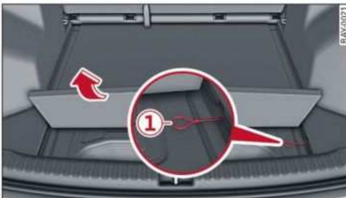
Fig. 83 Right side of the luggage compartment: charging connector manual emergency release
