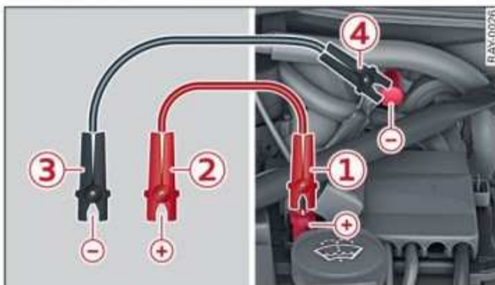
Fig. 167 Connecting the jump start cables
