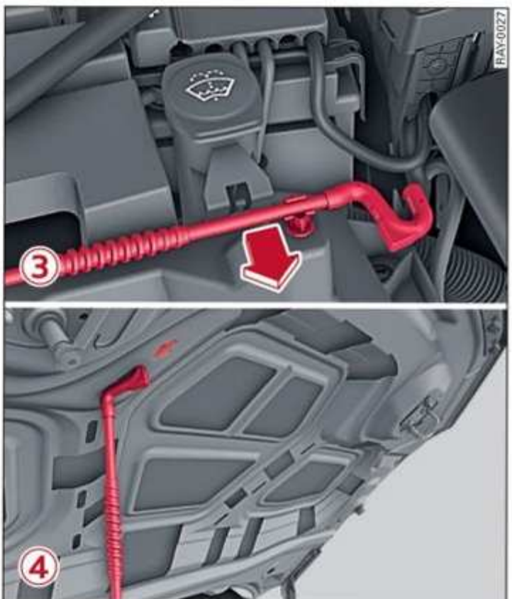
Fig. 150 ③ Front compartment: hood support in the re- tainer; ④ the hood support is inserted in the hood
