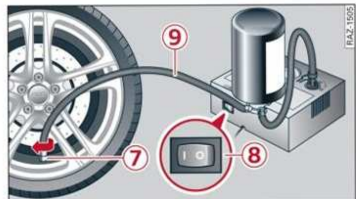
Fig. 163 Tire mobility kit connection
