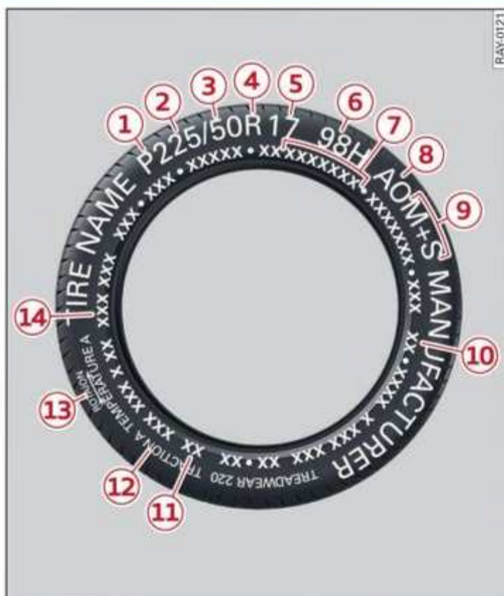
Fig. 156 Tire designations on the sidewall
