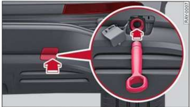
Fig. 170 Rear bumper: installing the towing loop
