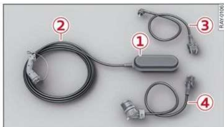
Fig. 87 Audi e-tron Charging System Compact: components (example)
