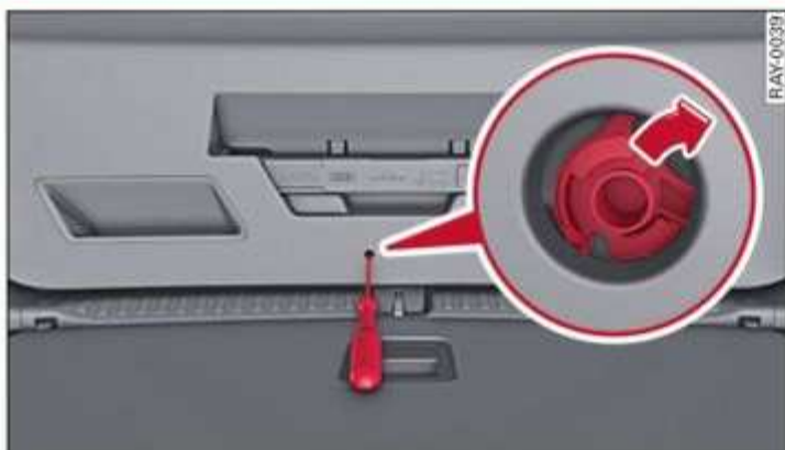
Fig. 33 Inner luggage compartment lid: access to the manual release
