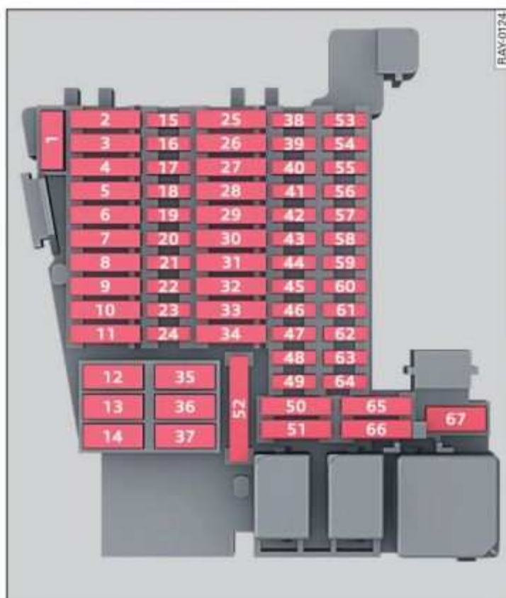
Fig. 173 Left side of cockpit: fuse assignment
