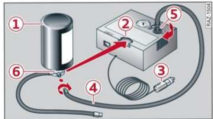
Fig. 162 Components of the tire mobility kit
