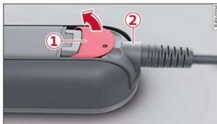
Fig. 89 Control unit: removing and attaching the cable
