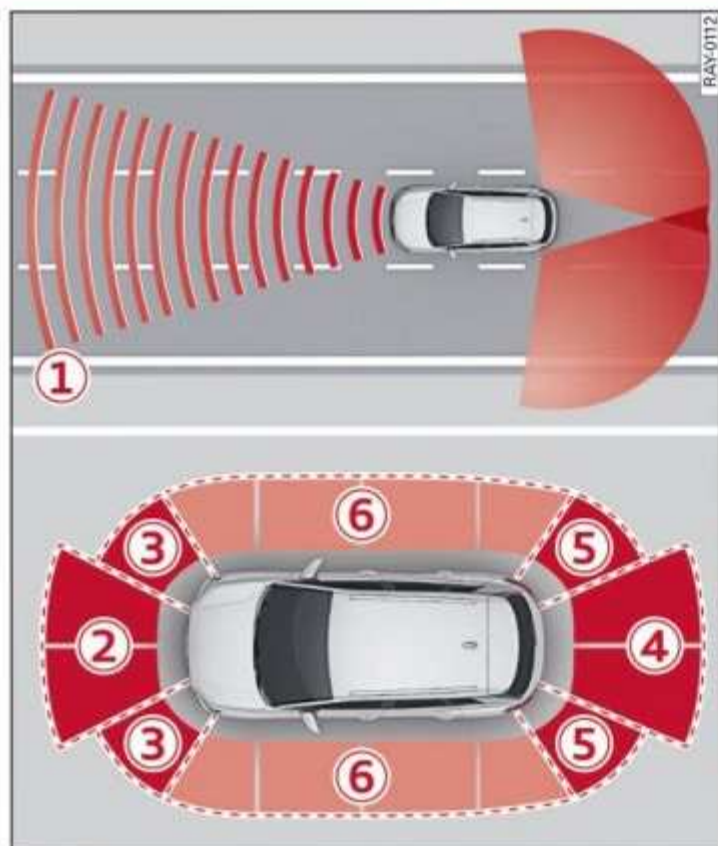
Fig. 92 Sensor detection ranges
