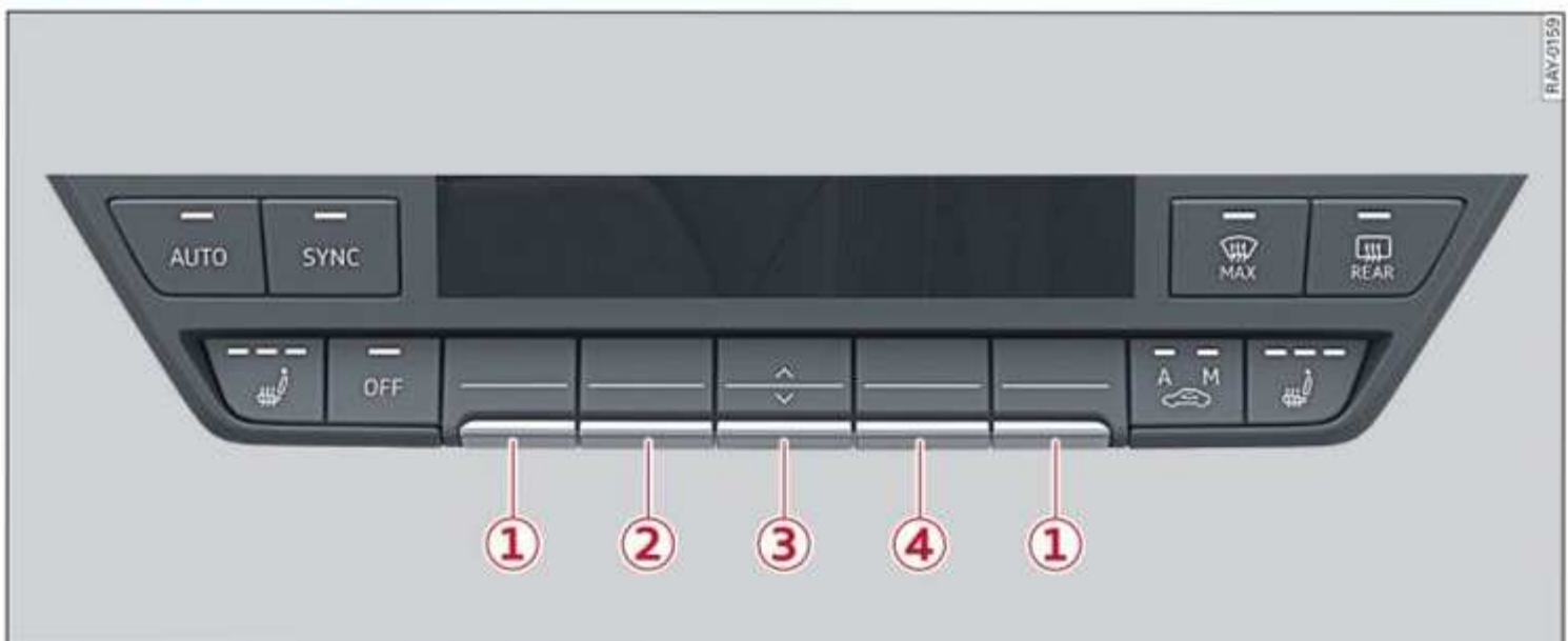
Fig. 76 Deluxe automatic climate control: controls
