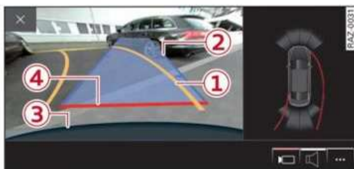
Fig. 123 Center display: aiming at a parking spot
