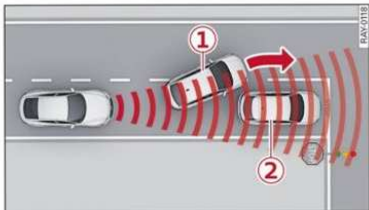
Fig. 101 Example: vehicle changing lanes and stationary vehicle
