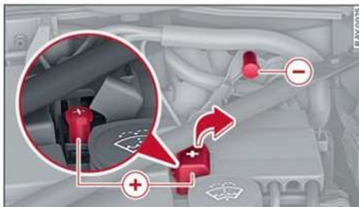
Fig. 154 Front compartment: connectors for a charger or jump start cables
