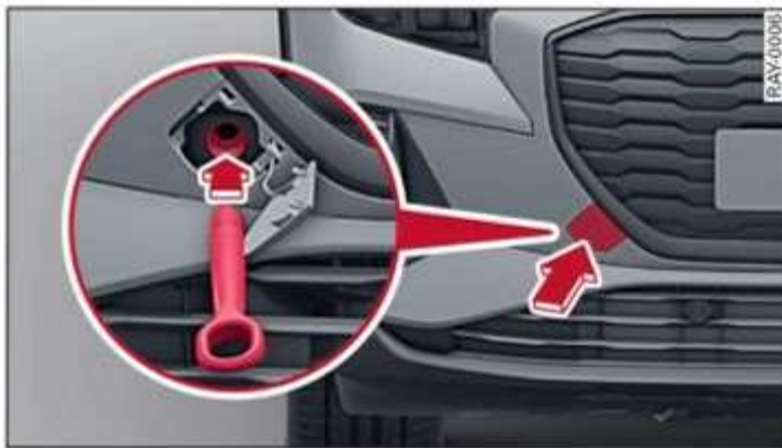
Fig. 169 Front bumper: installing the towing loop
