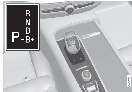
Overview of gear selector and gear shift pattern in the instrument panel.
