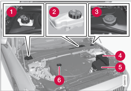
The layout of the engine compartment may vary depending on model and engine variant.
